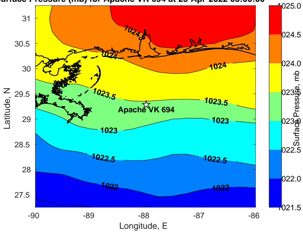
Surface Pressure (mb) for Apache VK 694 at 23-Apr-2022 03:00:00
